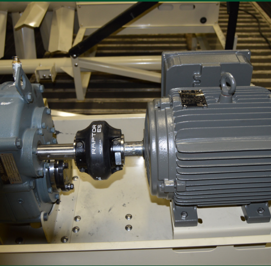
Direct-Drive Aerators
