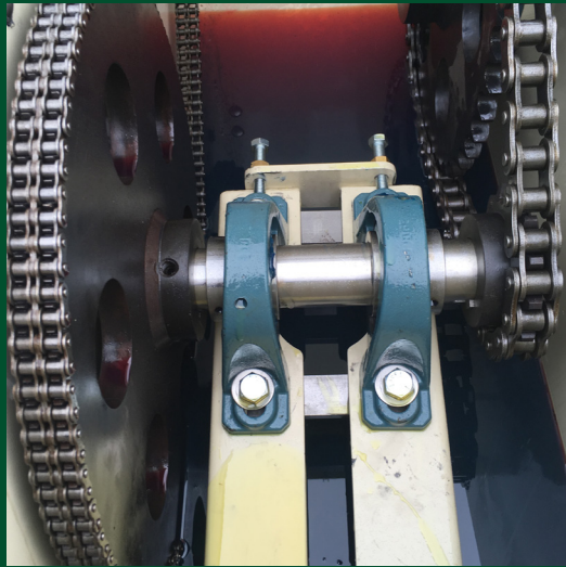
Chain-Drive Aerators
